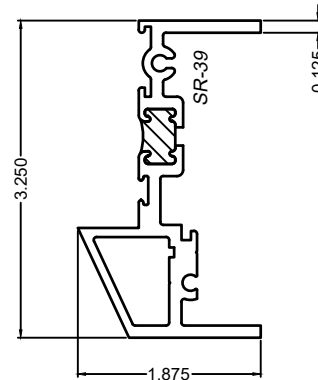
FRAME, FIXED, EXT. LEG AT MULLION - FX/AWN SR-39
