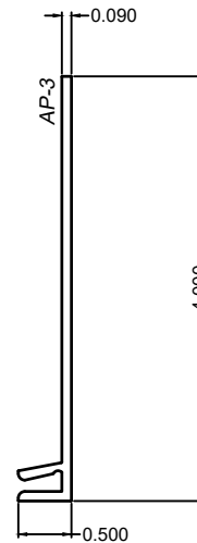
ANCHOR STRAP, F-CLIP, 1-1/2\"/>
