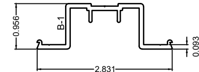
CLAMP, MULLION B-1
